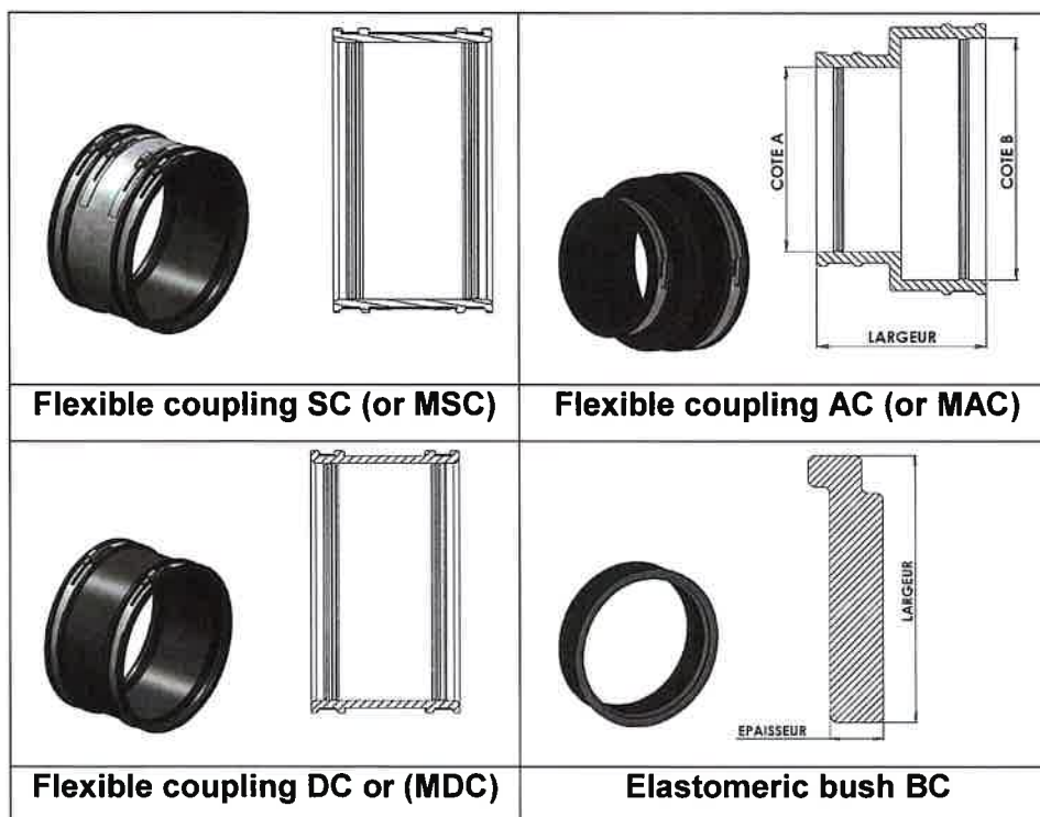
Figure 1 : Ranges of flexible couplings FLEX-SEAL Plus or CANADA Plus
